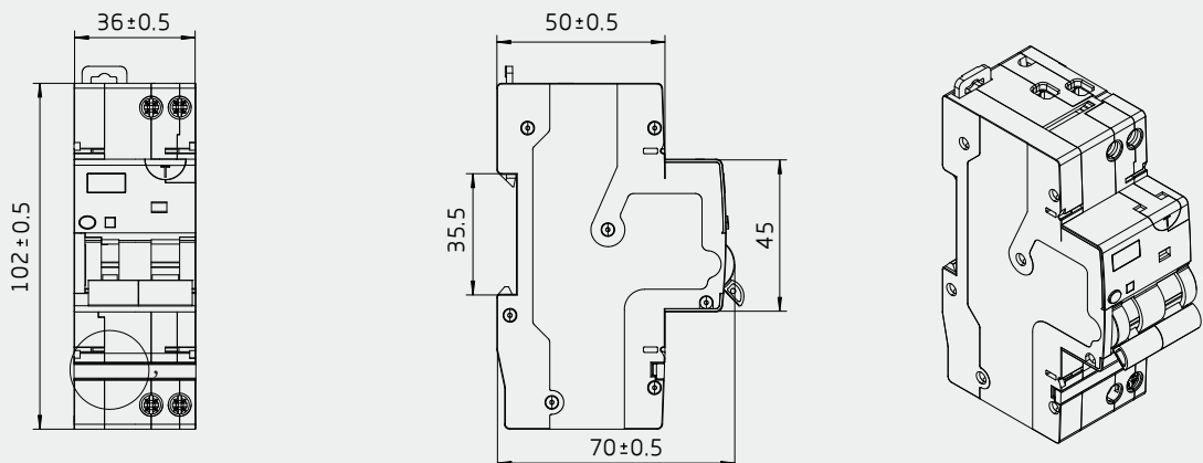
Product outline and installation dimension drawing (mm)
